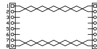
Main - Remote Interconnect 2 x Twisted pair
