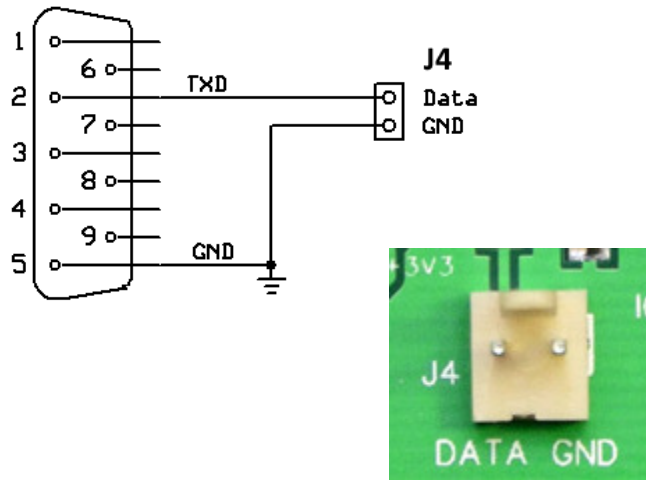
Figure 1 - RS-232 Connection
